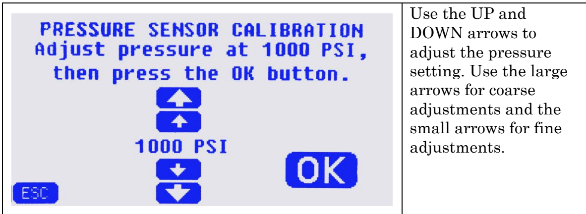
Figure 18 – Adjusting pressure at max pressure.
