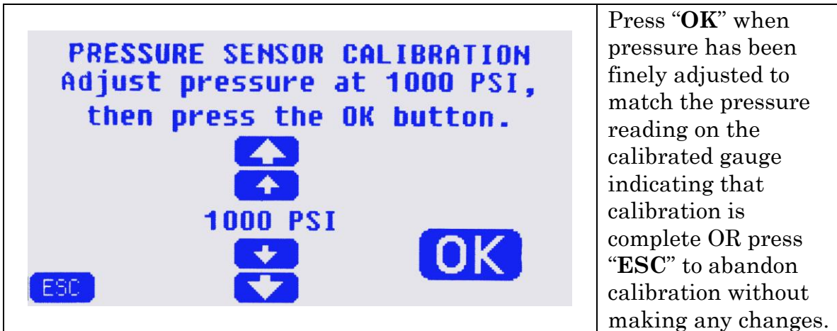
Figure 19 – Completing the calibration.
