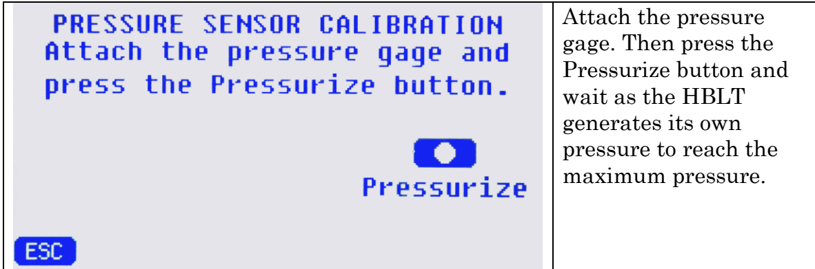
Figure 16 – Pressurizing the HBLT.
